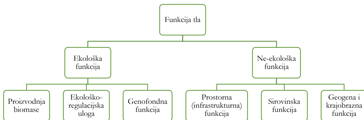
Slika 4.37 Funkcije tla (Izvor: Functions of soil for society and the environment, 2005)
